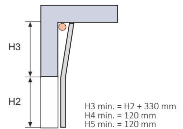
VERTICAL IND-VL
