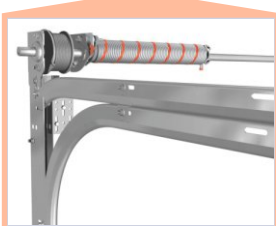
RES200 Linteau Normal (RESSORT AVANT)
